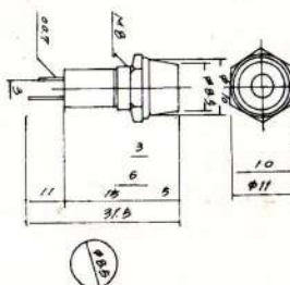
L-607 LED INDICATOR LIGHT w o resistor 2V
