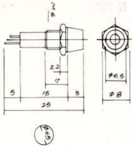
L-608 LED INDICATOR LIGHT w o resistor 2V
